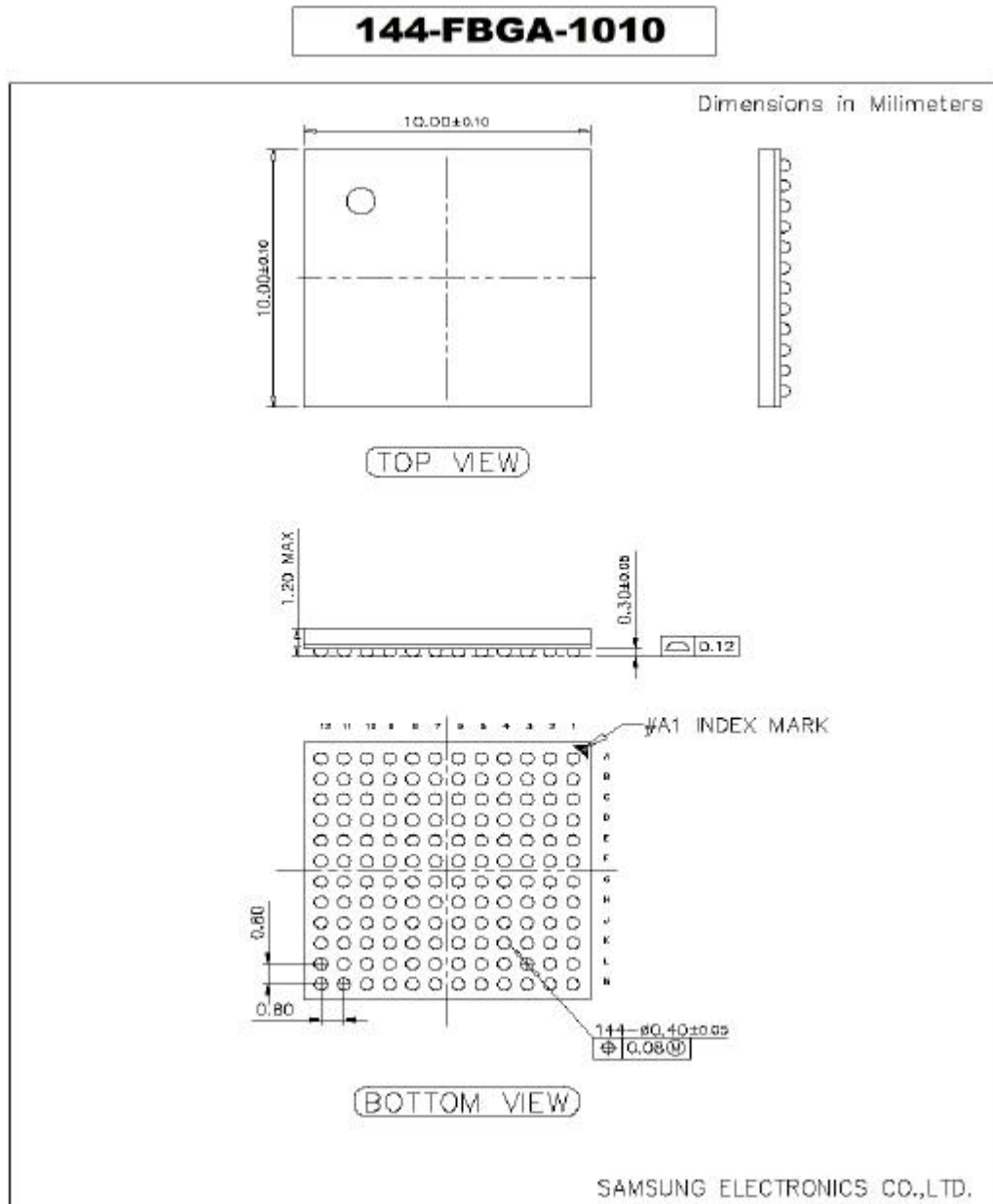
Figure 15-1. 144-FBGA-10.0X10.0 Package Dimension
